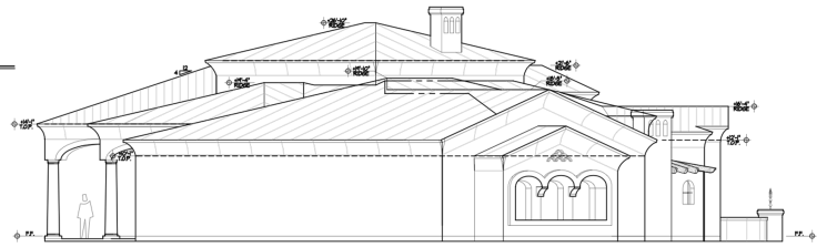
LEFT ELEVATION (7516 PLAN)
