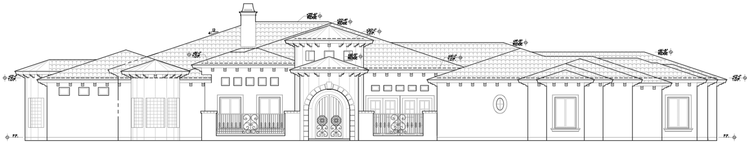
NORTH COURT-YARD ELEVATION (5483 PLAN)
